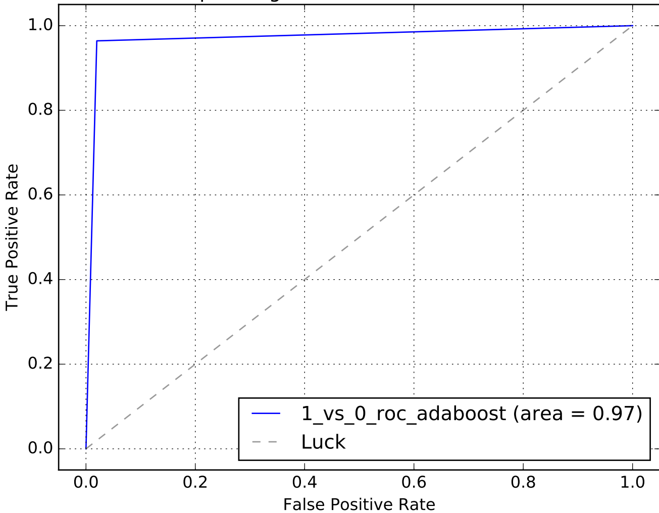
Receiver operating characteristic N0=7606, N1=4159
