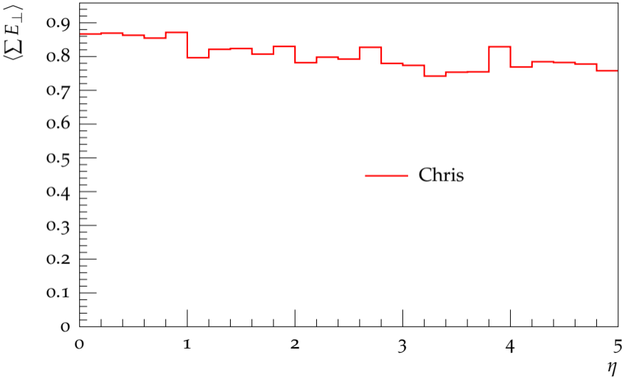
Pseudorapidity distribution of \langle \Sigma E_{\perp} \rangle
