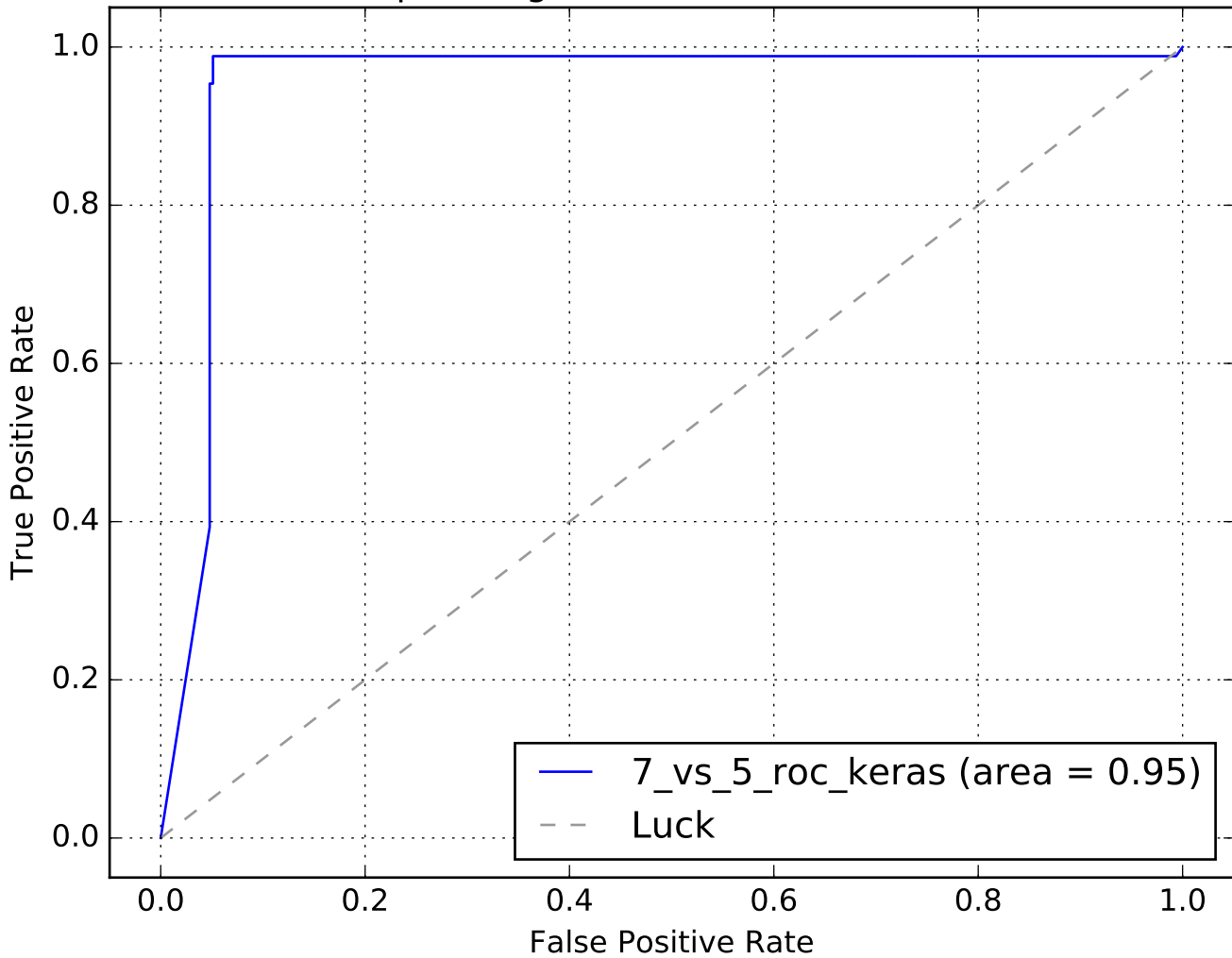
Receiver operating characteristic N0=611, N1=361
