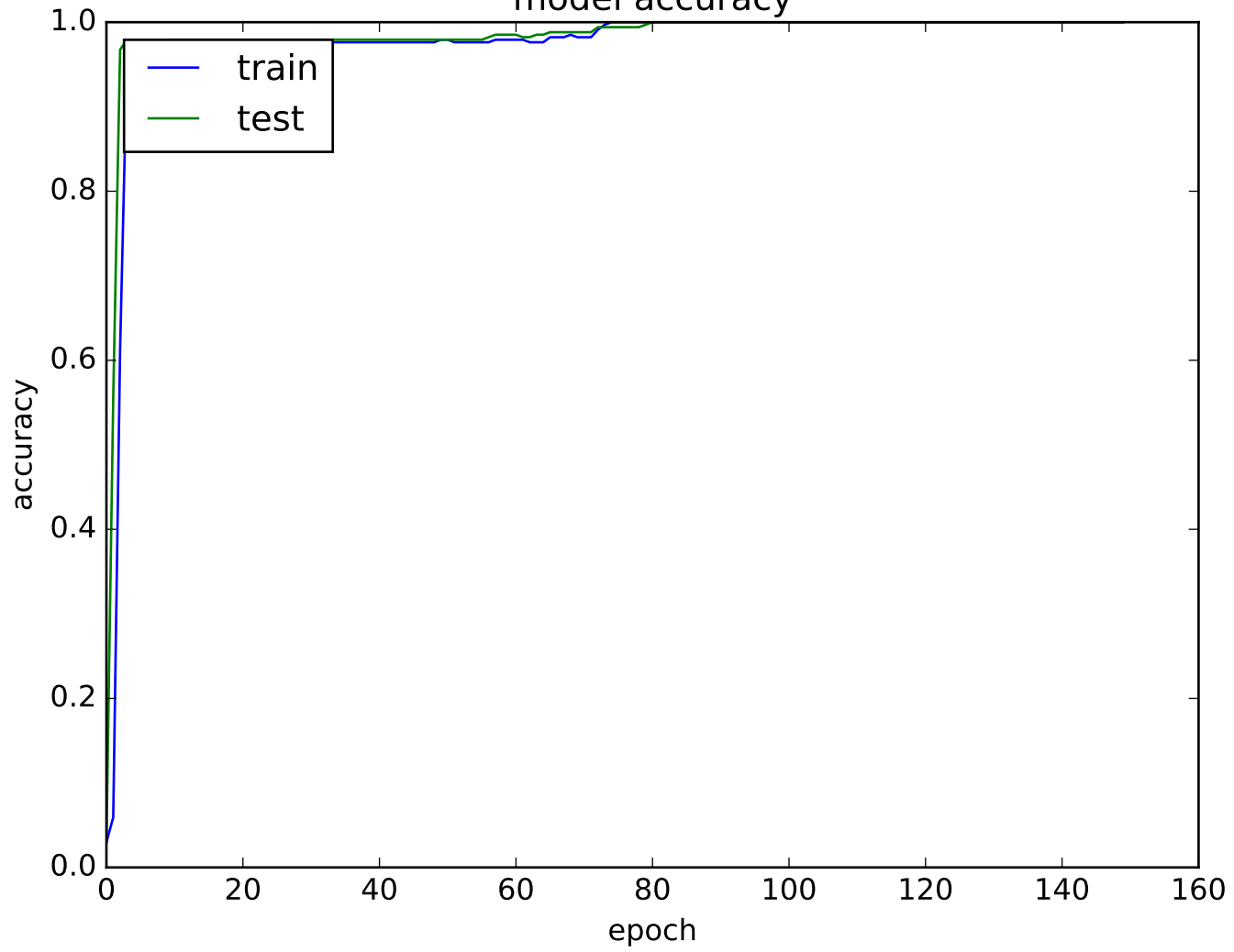
model accuracy
