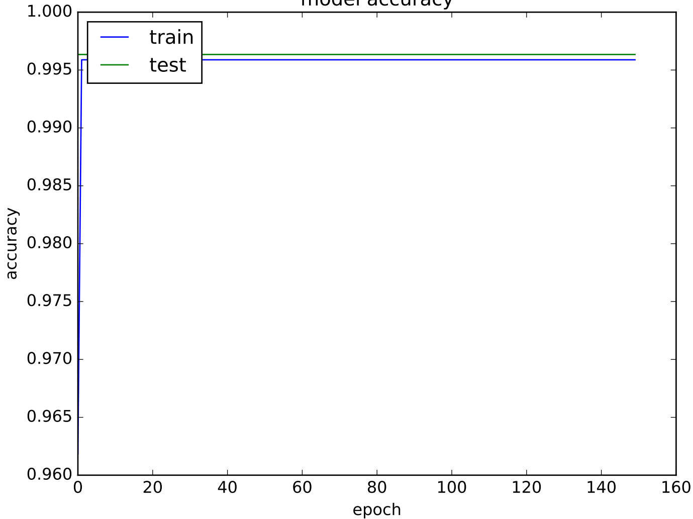
model accuracy
