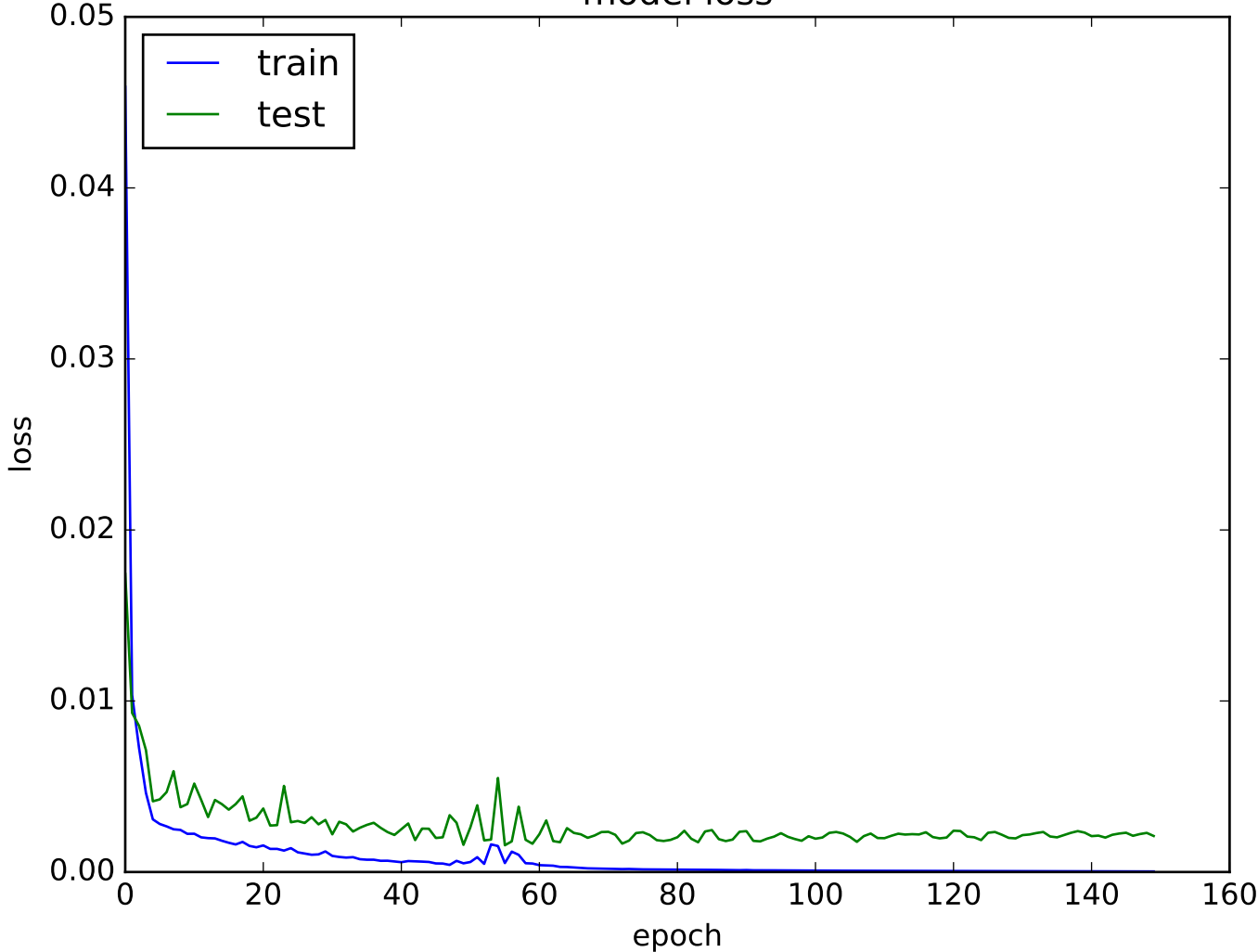
model loss
