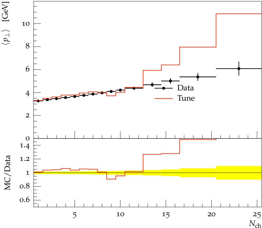
Charged \langle p_{\perp} \rangle vs. N_{\text{ch}} at 7 TeV, track p_{\perp} > 2500 MeV, for N_{\text{ch}} \geq 1
