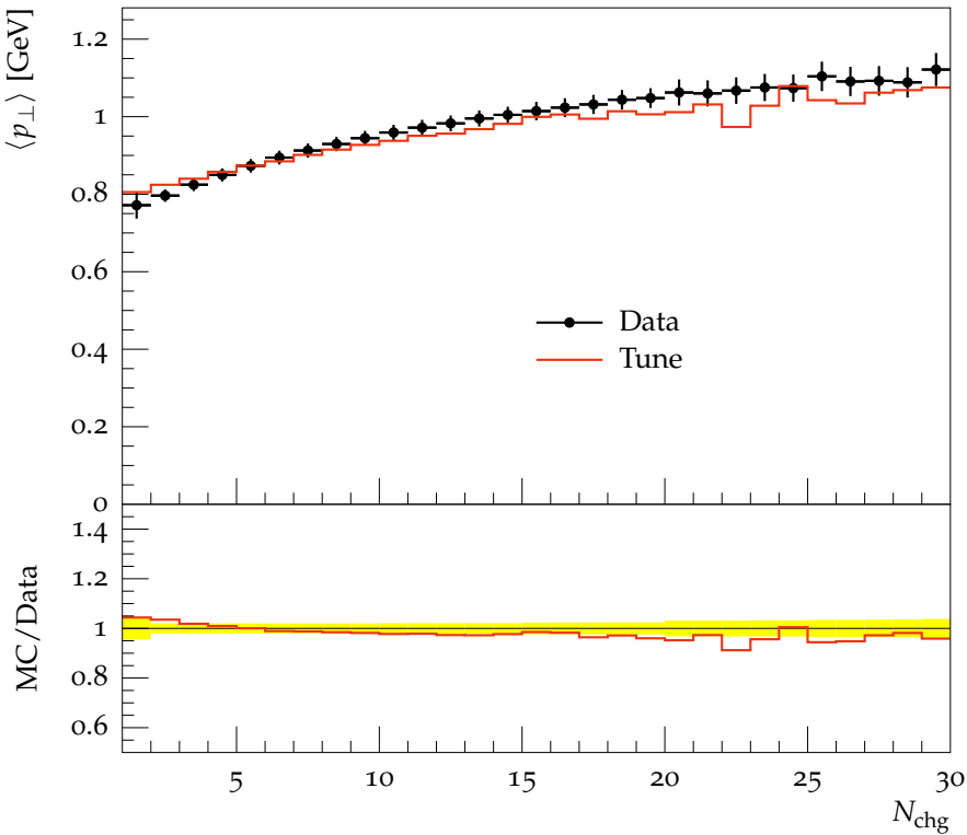
Away \langle p_{\perp} \rangle vs. N_{\text{chg}} , \sqrt{s} = 7 TeV
