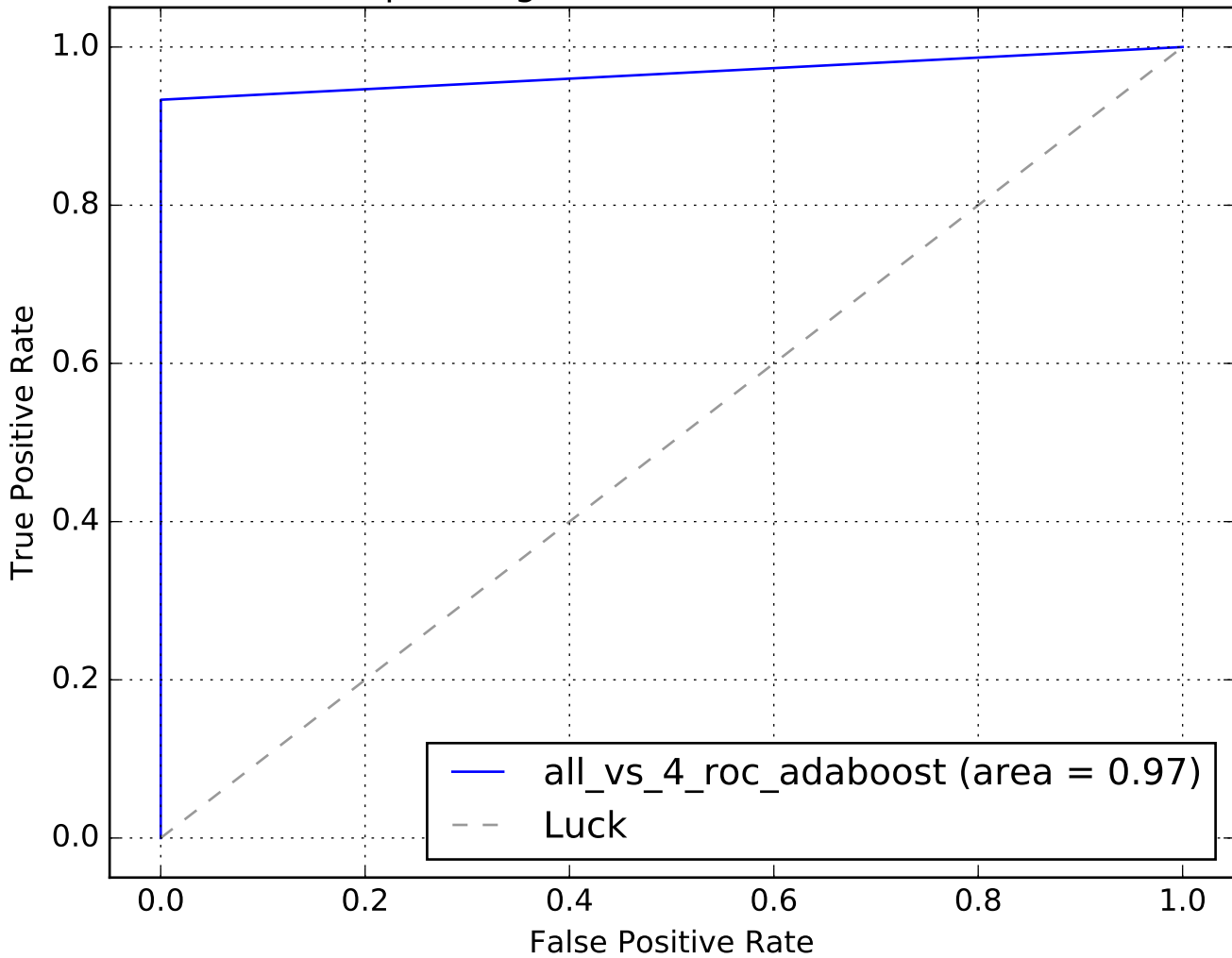
Receiver operating characteristic N0=17432, N1=64
