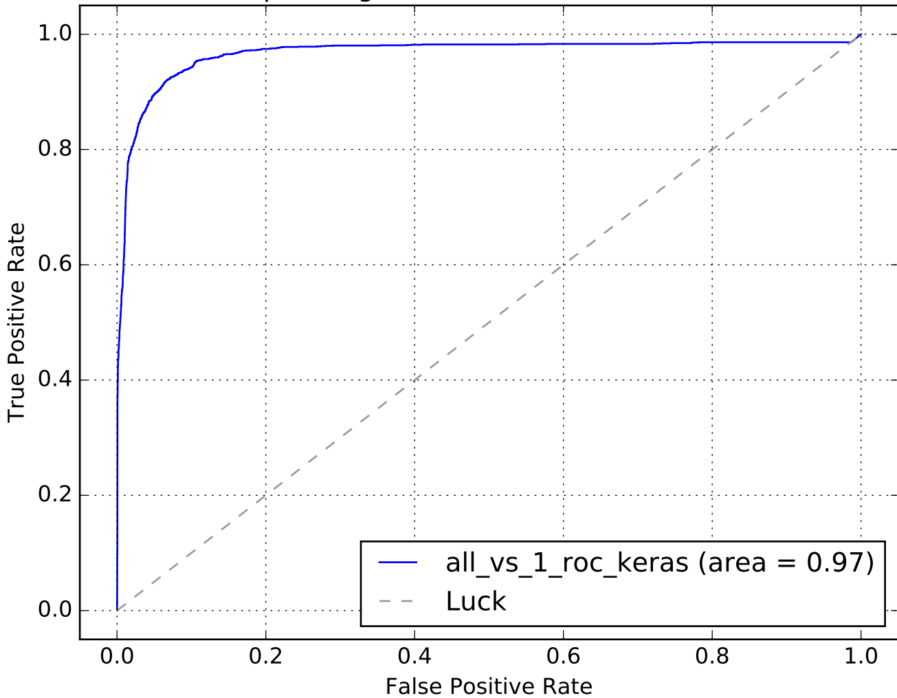
Receiver operating characteristic N0=13337, N1=4159
