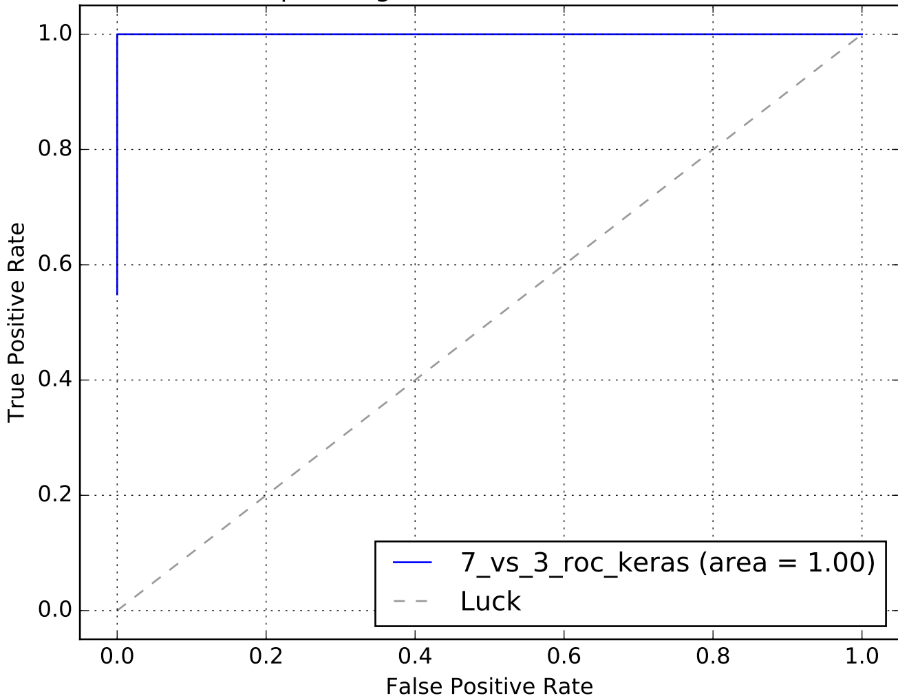
Receiver operating characteristic N0=3344, N1=361
