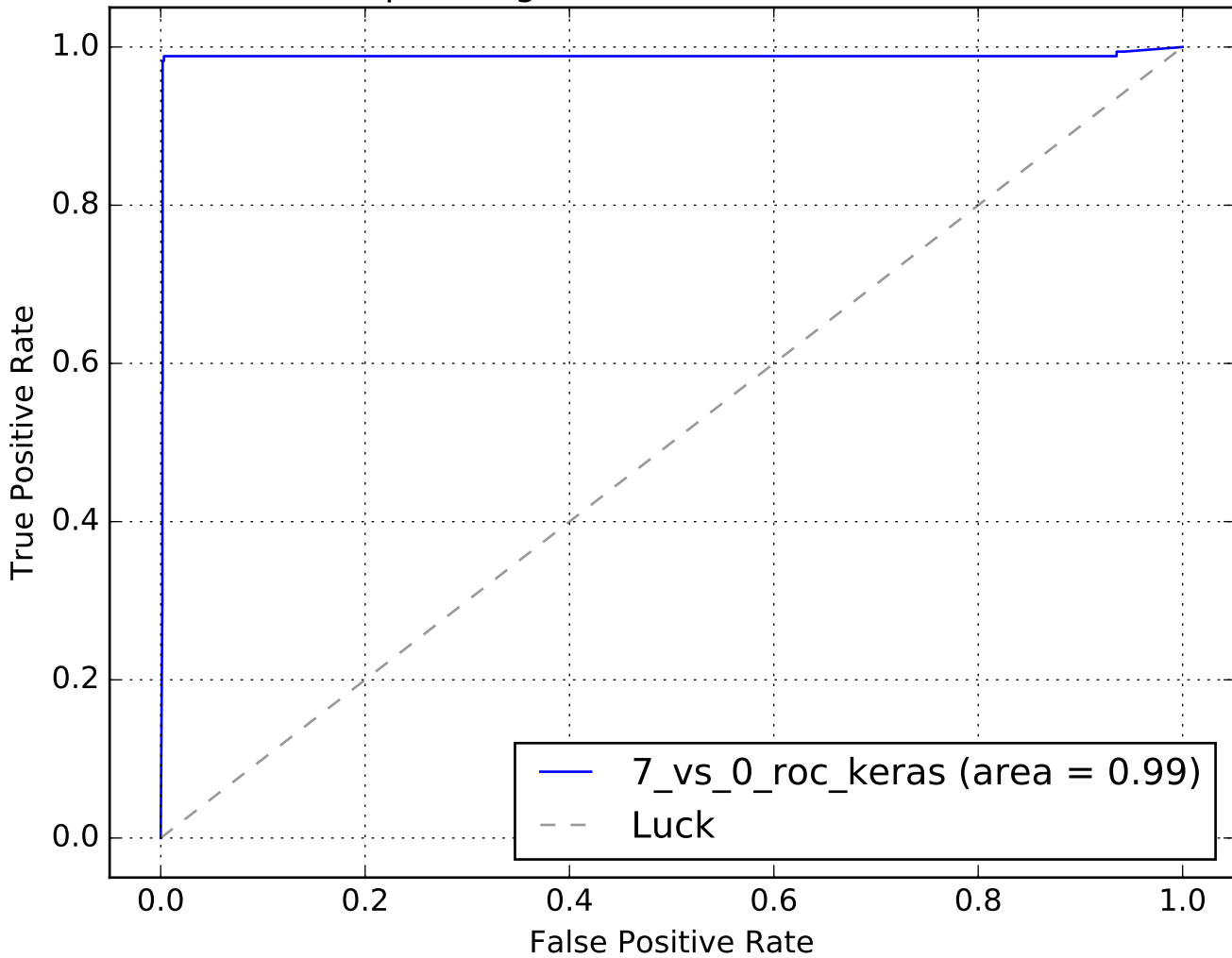
Receiver operating characteristic N0=7606, N1=361
