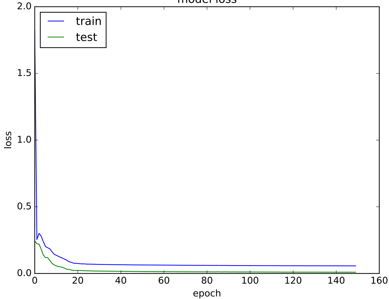
model loss
