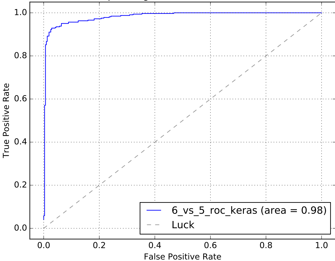
Receiver operating characteristic N0=611, N1=665
