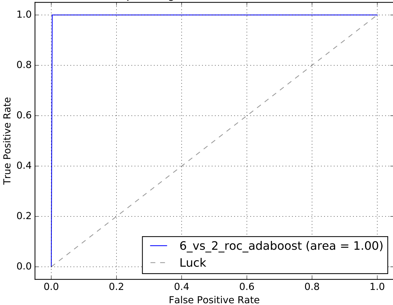
Receiver operating characteristic N0=686, N1=665
