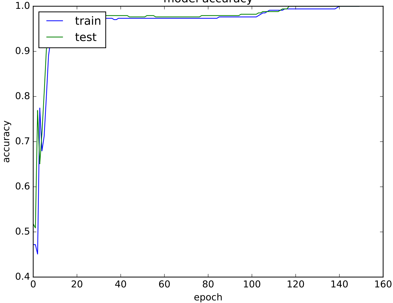
model accuracy
