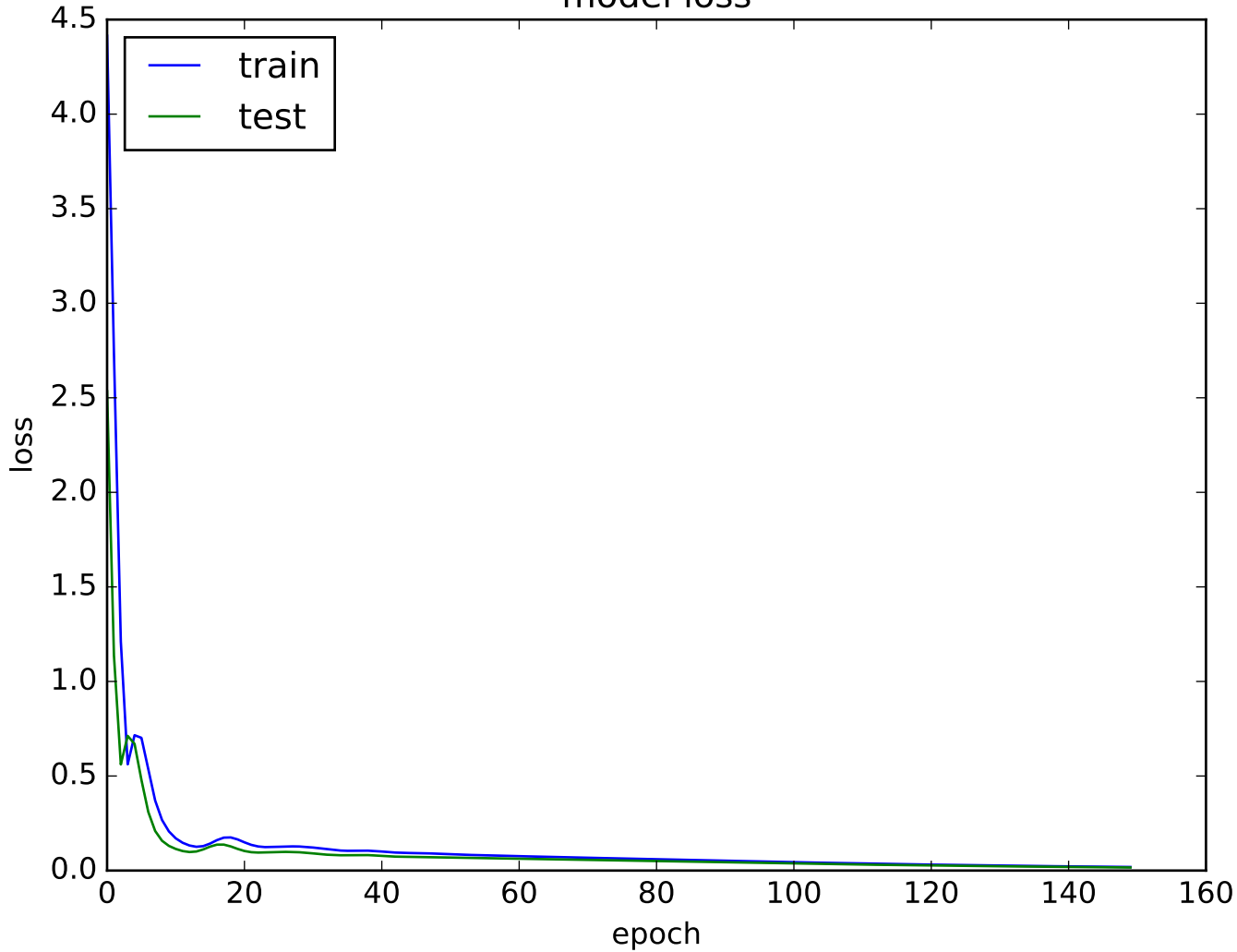
model loss
