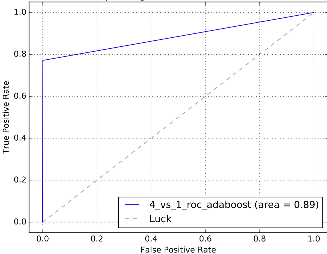
Receiver operating characteristic N0=4159, N1=64
