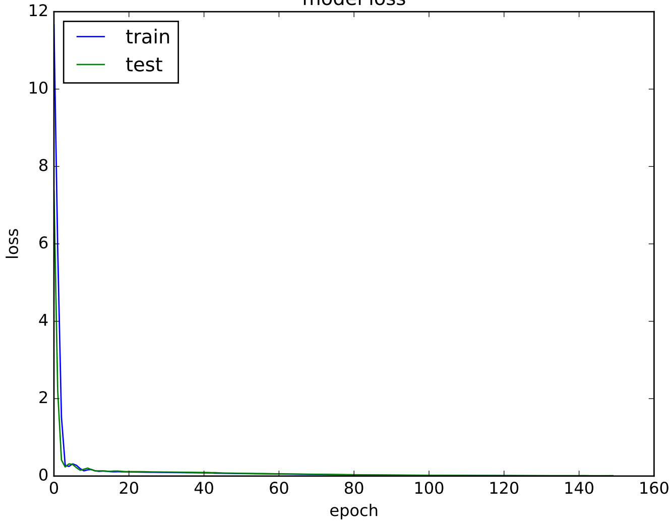
model loss
