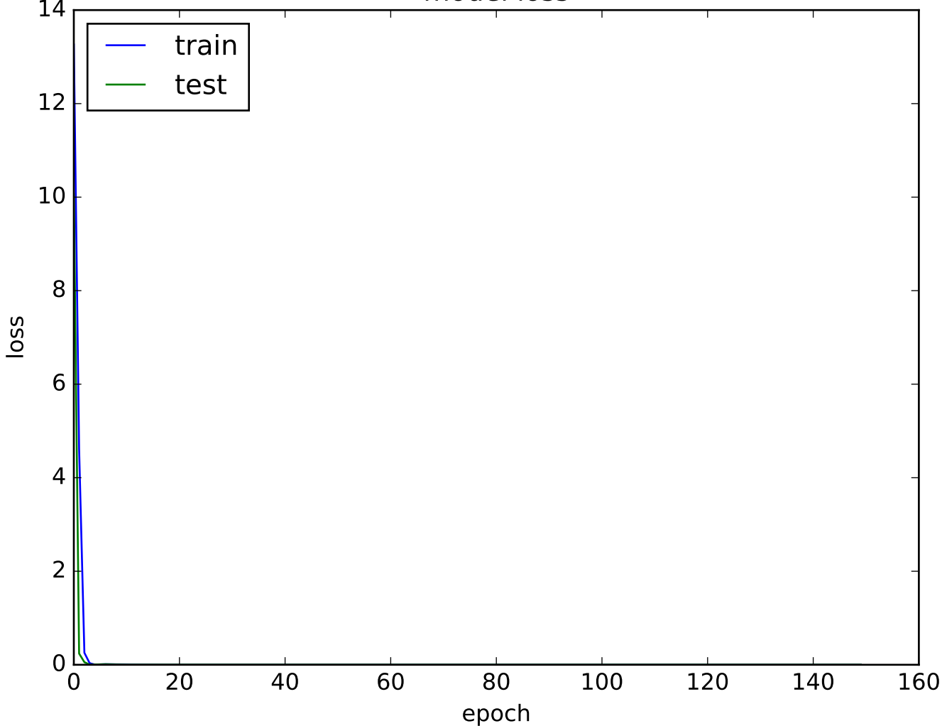
model loss
