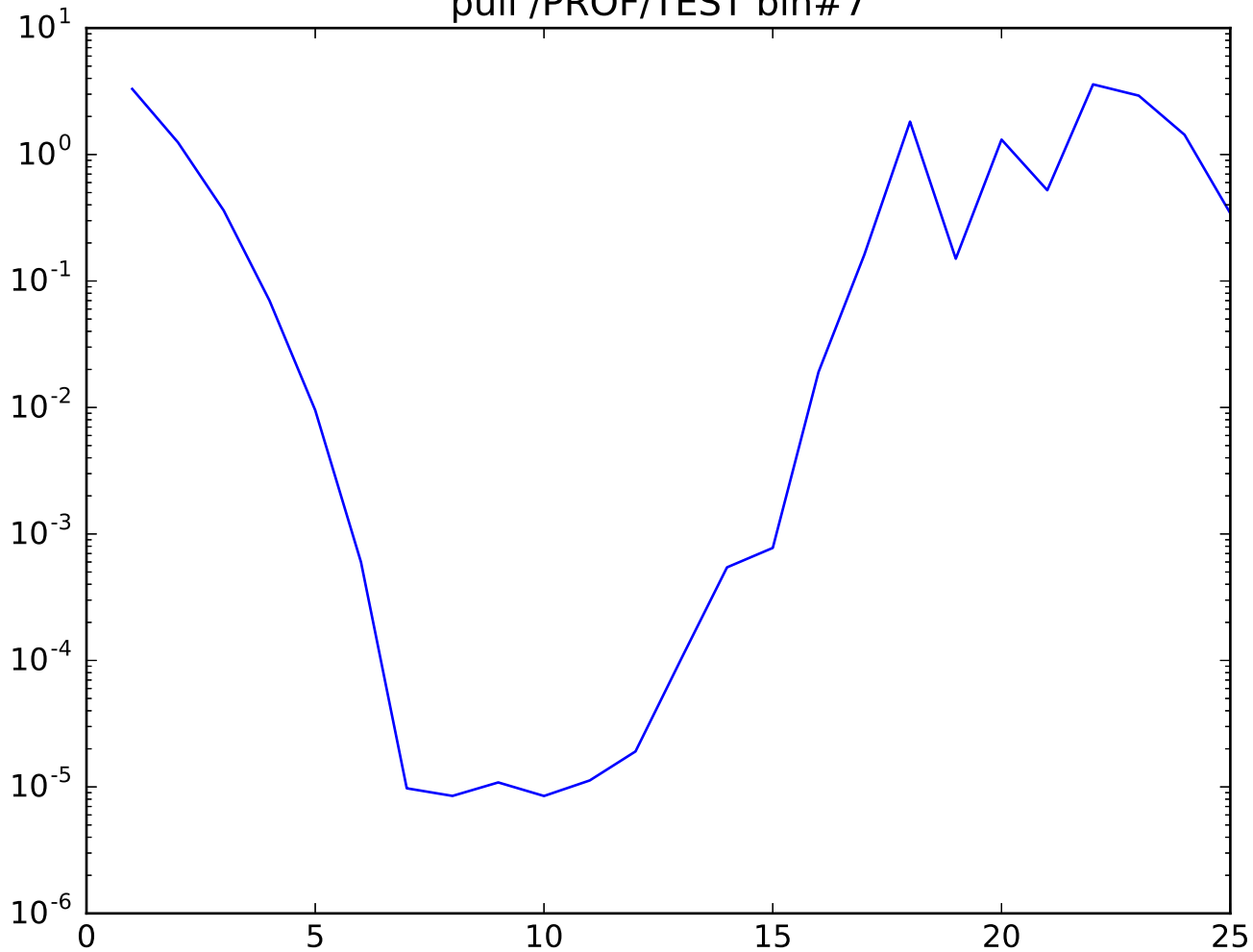
pull /PROF/TEST bin#7
