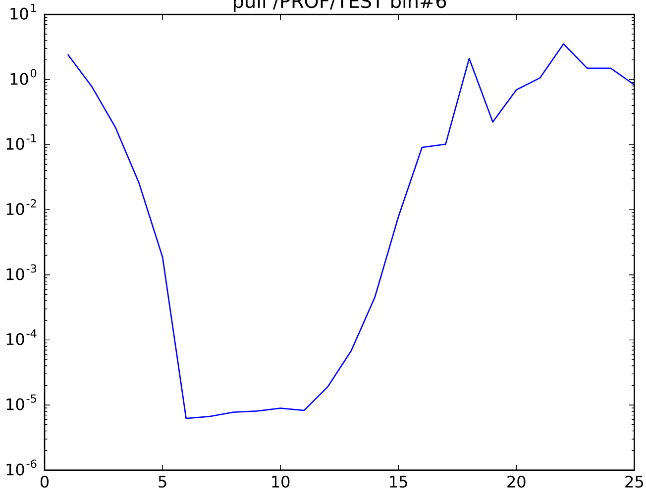
pull /PROF/TEST bin#6
