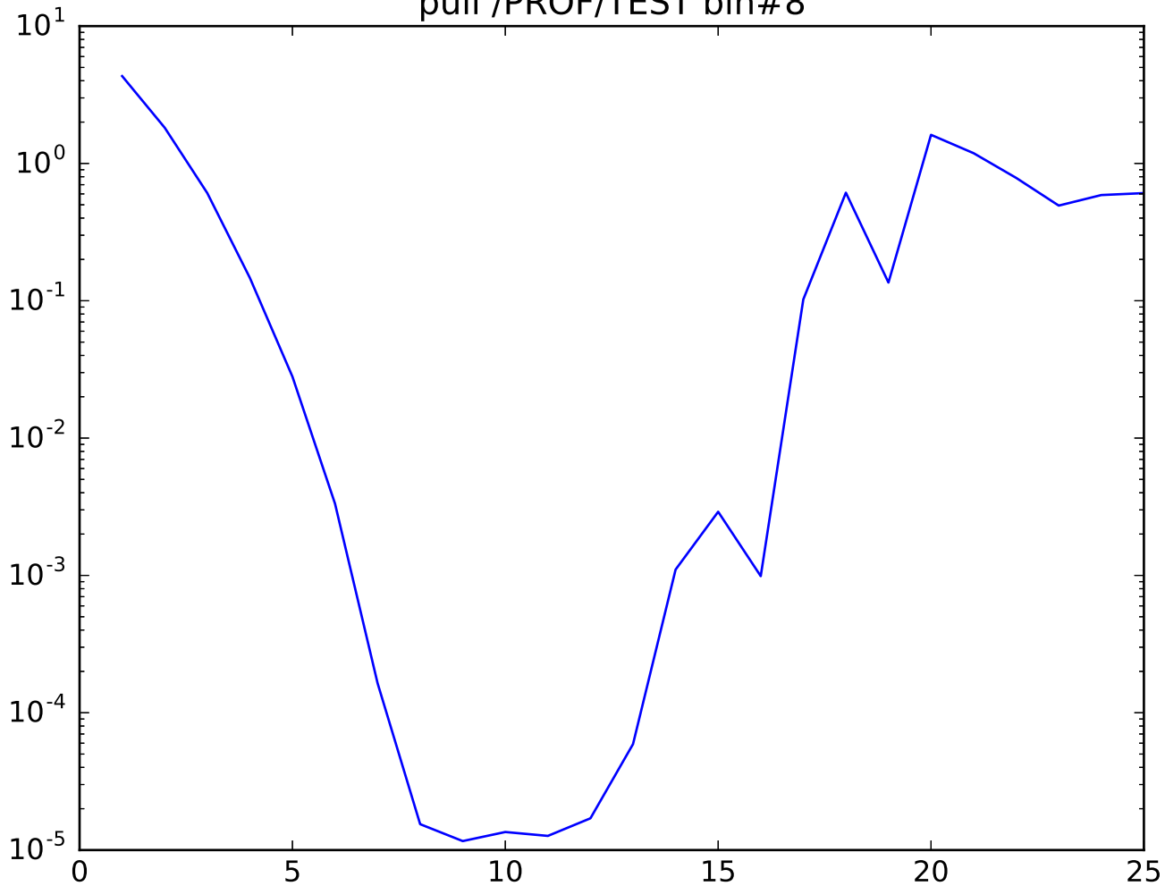
pull /PROF/TEST bin#8
