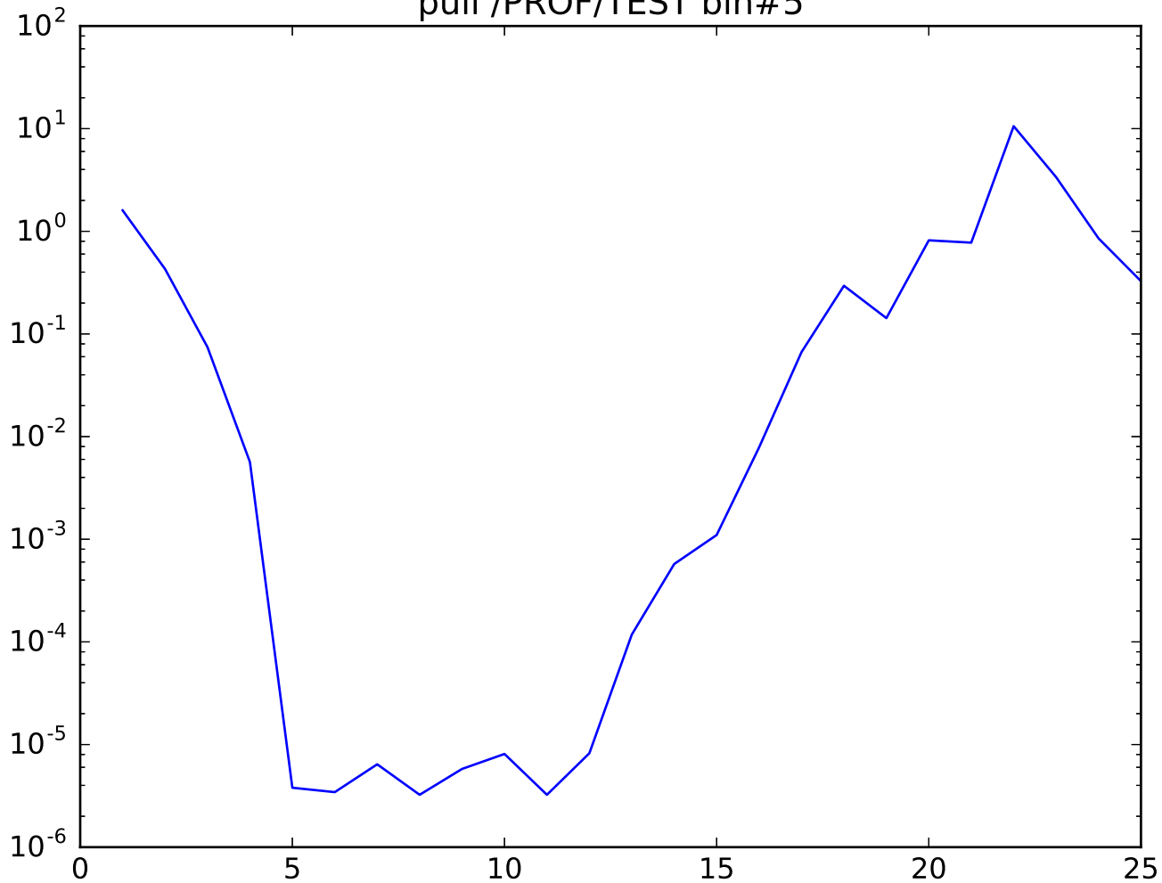
pull /PROF/TEST bin#5
