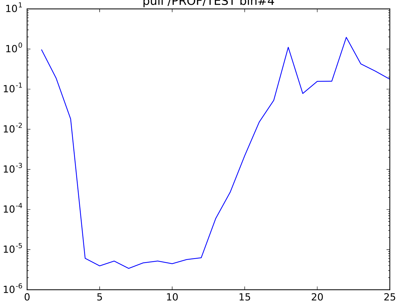
pull /PROF/TEST bin#4
