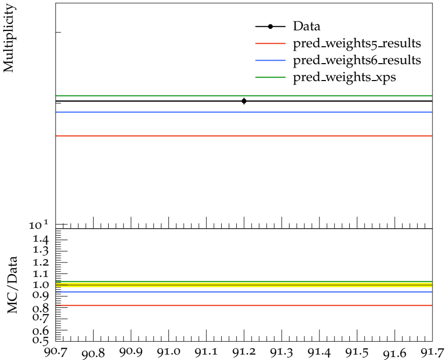
uds events mean charged multiplicity
