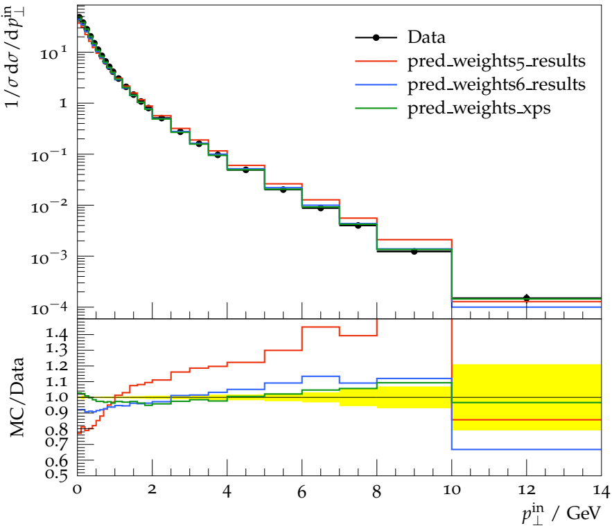
In-plane p_T in GeV w.r.t. sphericity axes (charged)
