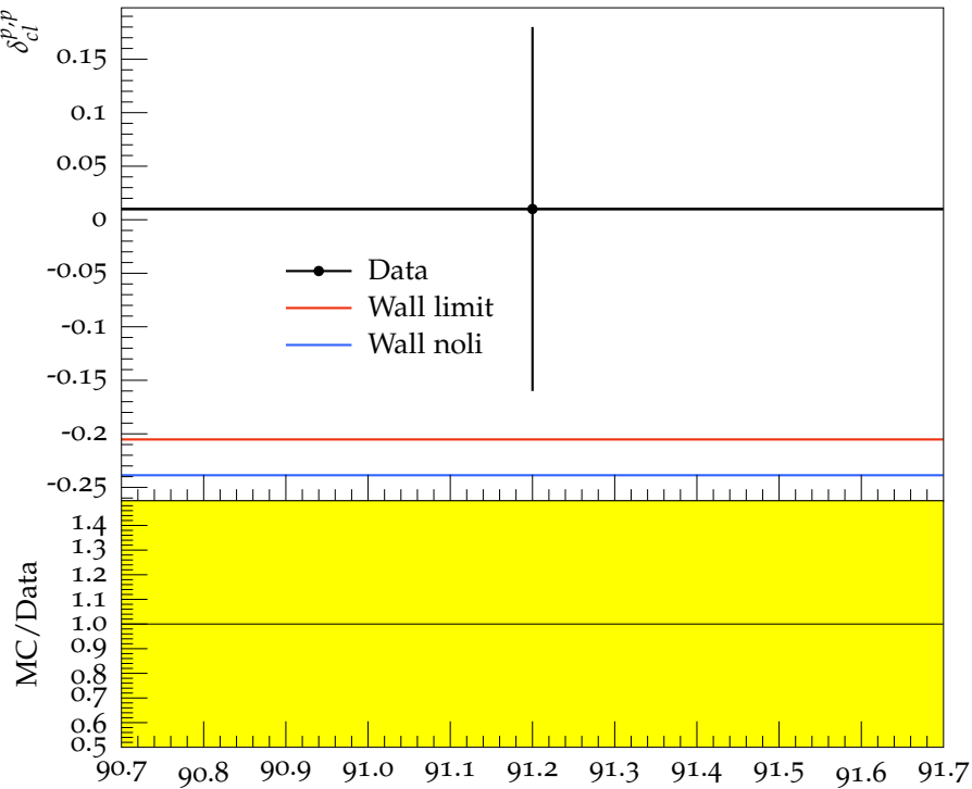
Multiplicity difference c -uds for p, \bar{p}
