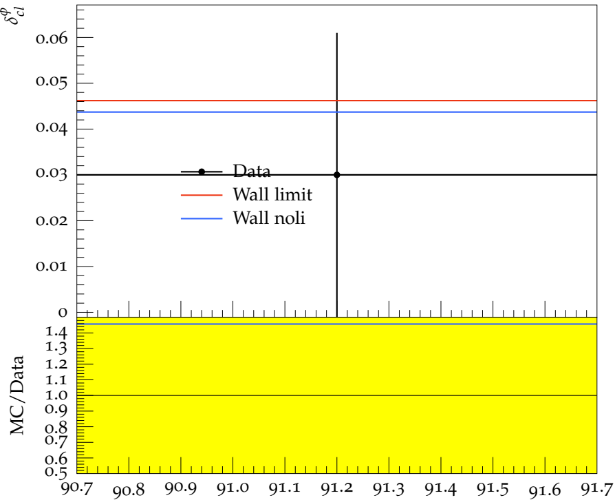
Multiplicity difference b -uds for \phi
