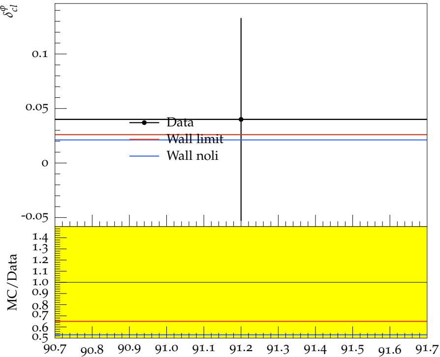
Multiplicity difference c - uds for \phi
