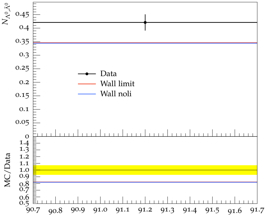
Multiplicity of \Lambda^0, \bar{\Lambda}^0 in ( uds ) events
