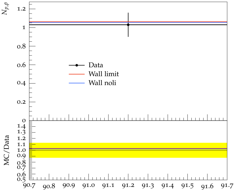
Multiplicity of p, \bar{p}
