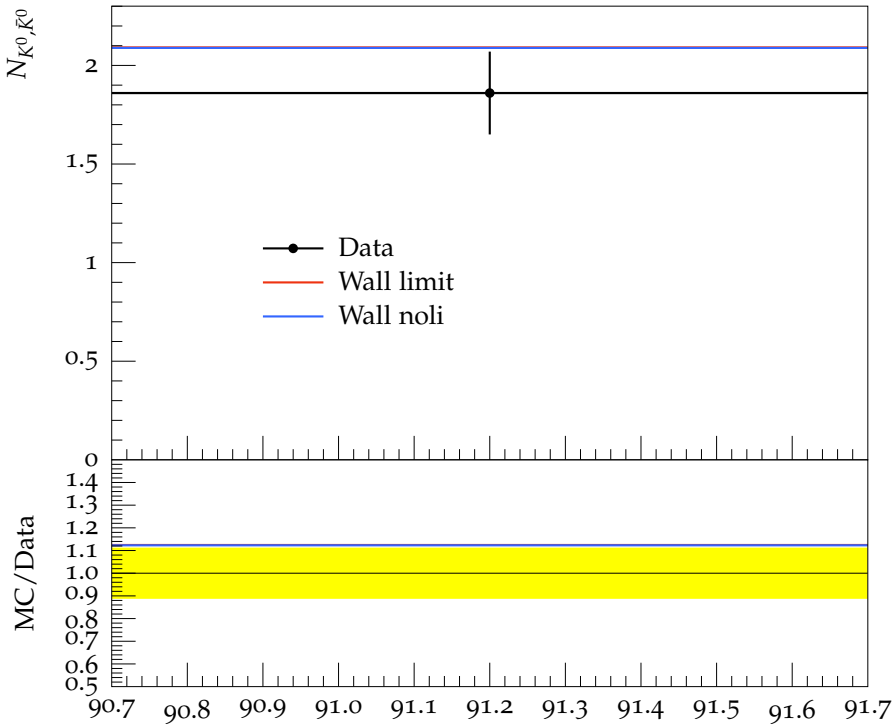
Multiplicity of K^0, \bar{K}^0 in c events
