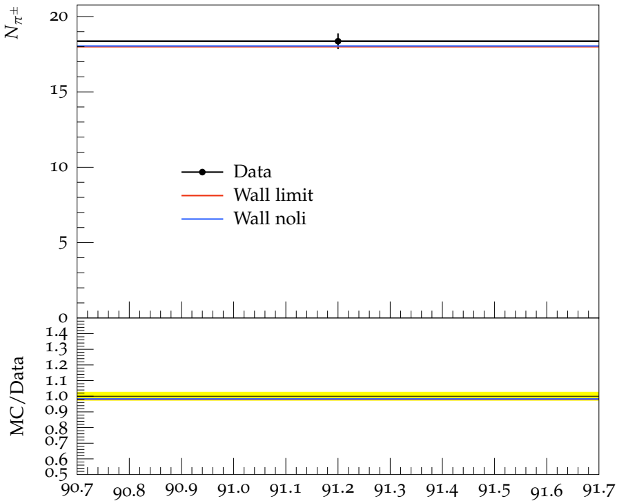
Multiplicity of \pi^\pm in b events
