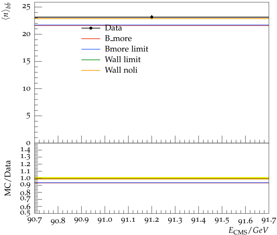
Charged multiplicity in b events
