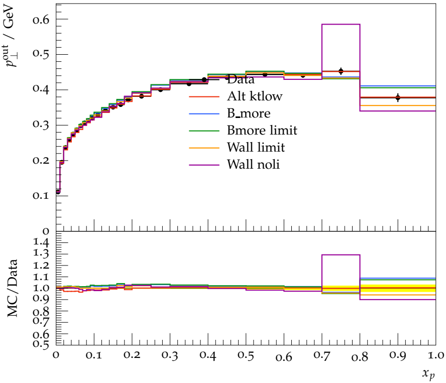
Mean out-of-plane p_{\perp} in GeV w.r.t. thrust axes vs. x_p
