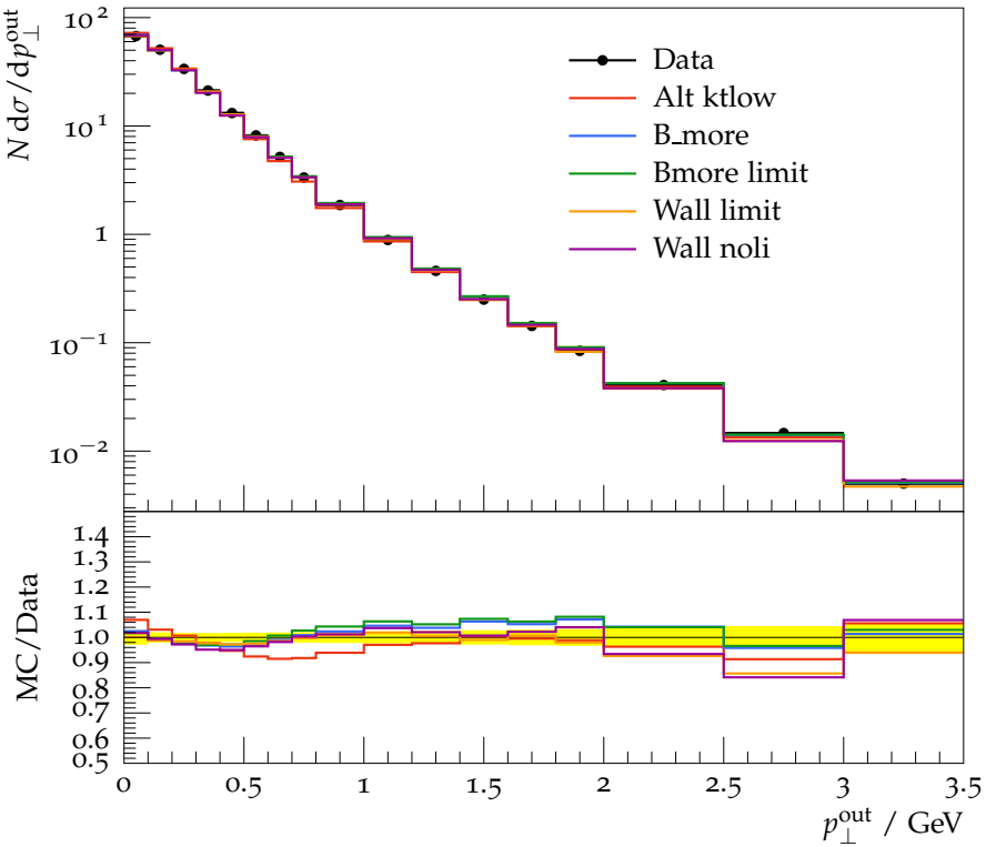
Out-of-plane p_{\perp} in GeV w.r.t. thrust axes
