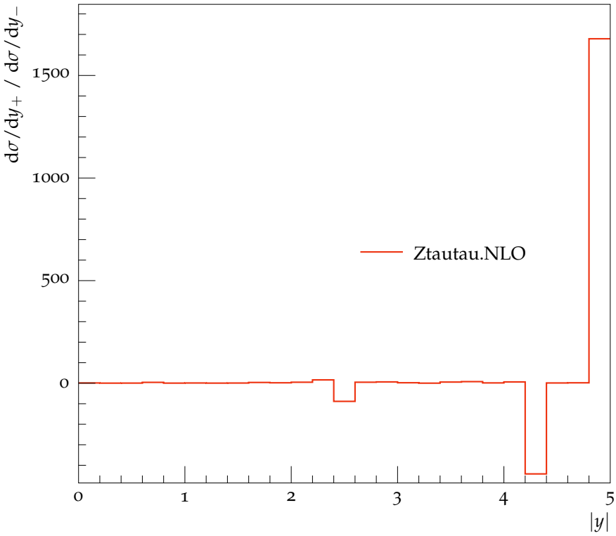
Rapidity +/- ratio of all particles
