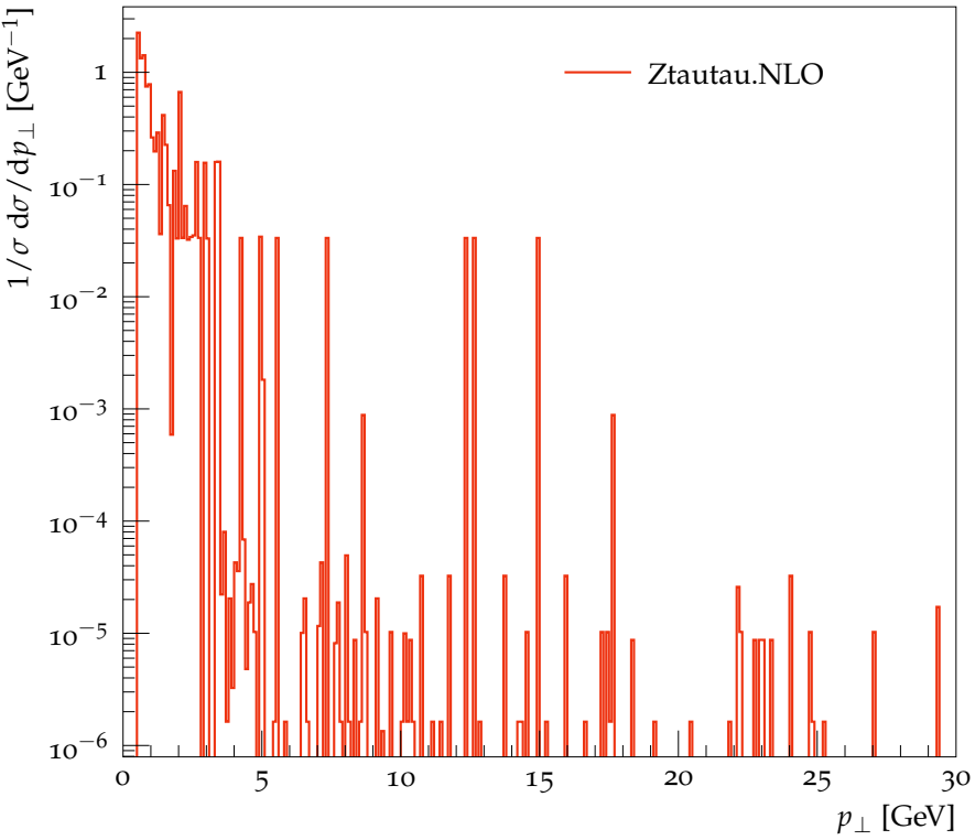
Transverse momentum of all particles
