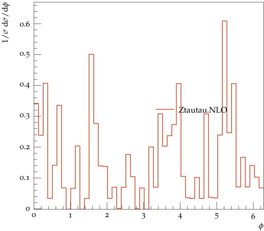
Azimuthal distribution of charged particles
