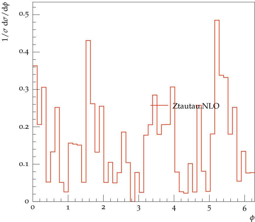
Azimuthal distribution of all particles
