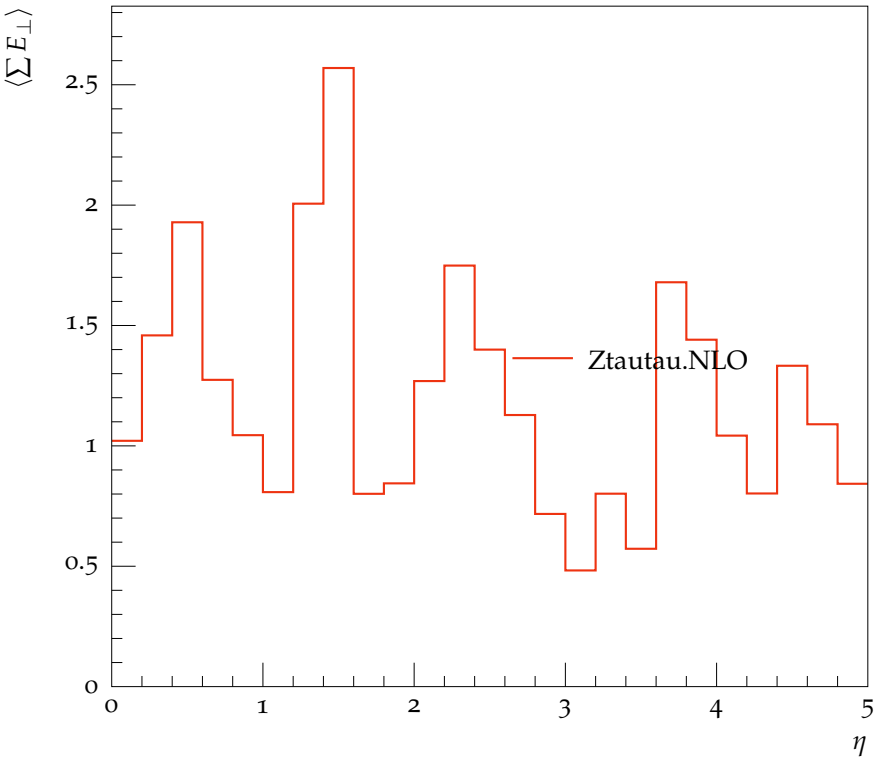
Pseudorapidity distribution of \langle \sum E_{\perp} \rangle
