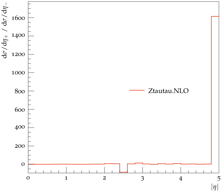
Pseudorapidity +/- ratio of all particles
