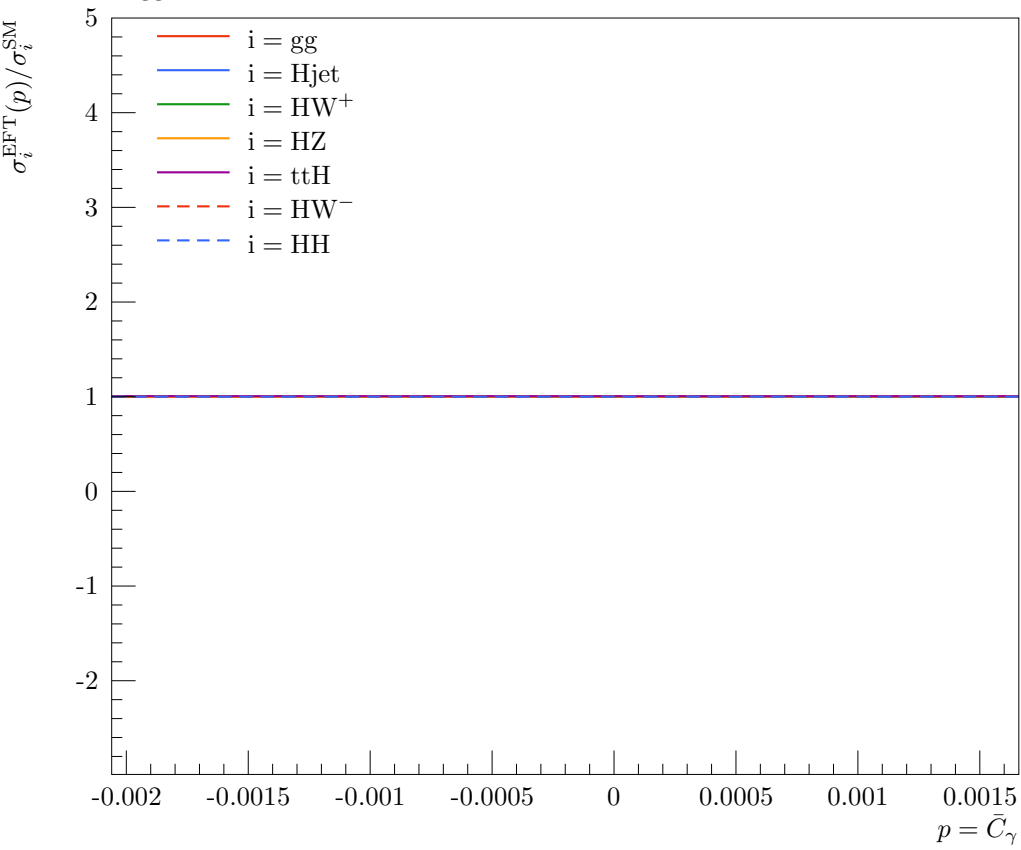
Higgs XS EFT over SM ratio scan
