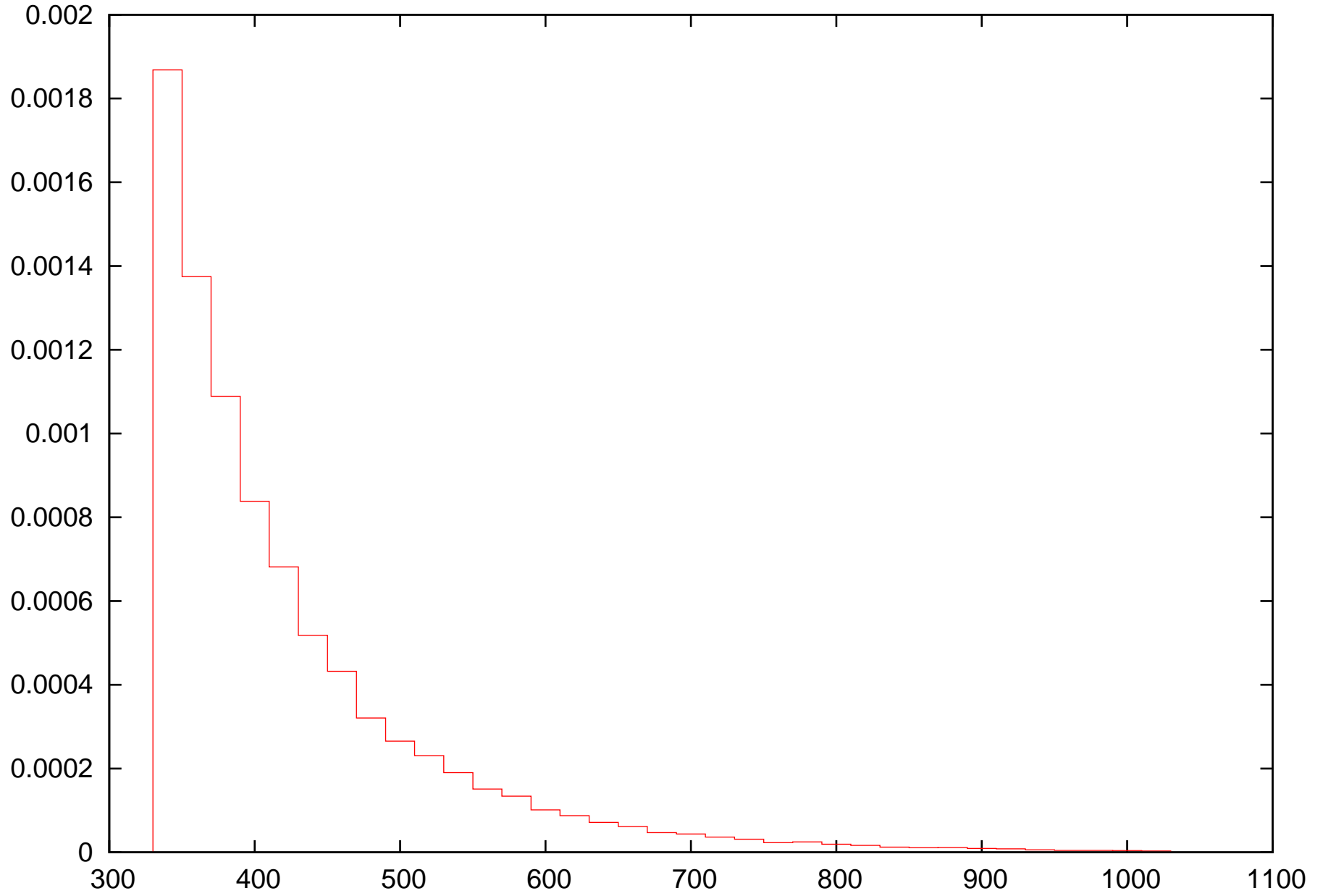
dS/dmZZ (fb/GeV)
