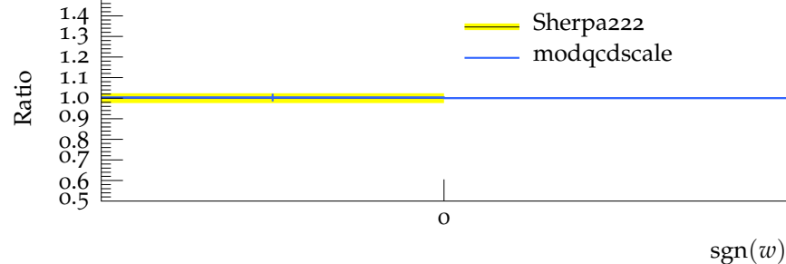
Fraction of positive and negative weighted events
