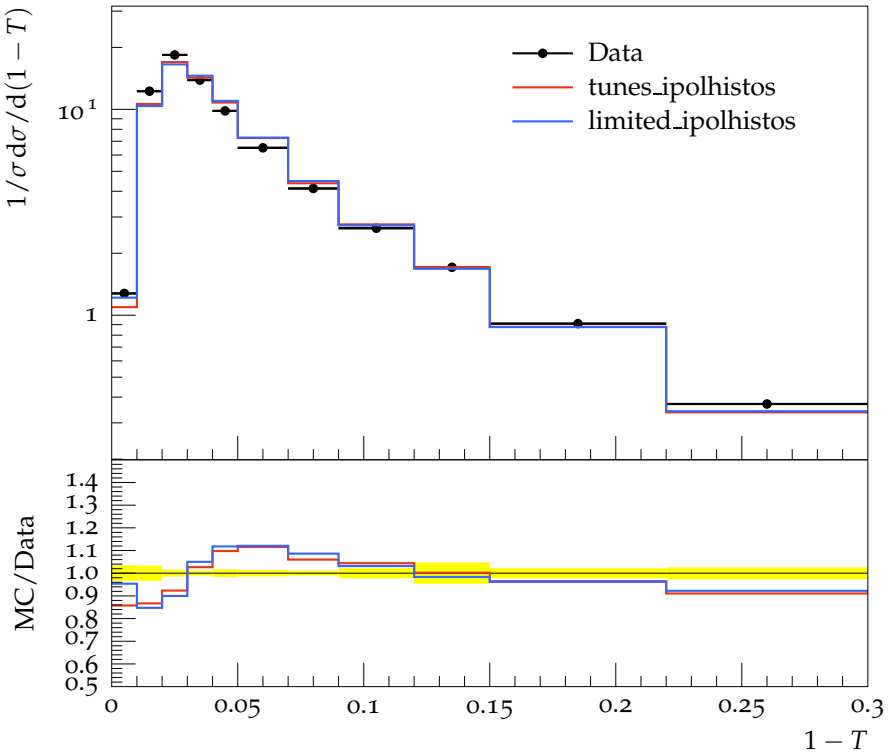
Thrust, 1 - T , at 91 GeV
