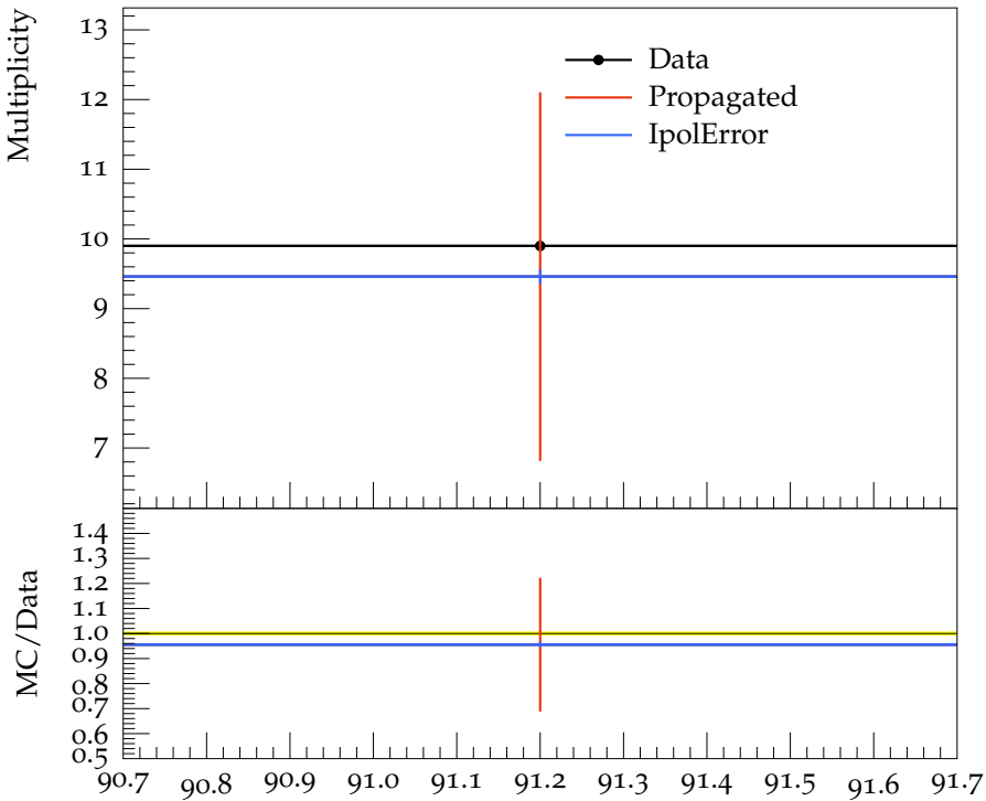
Mean \pi^0 multiplicity
