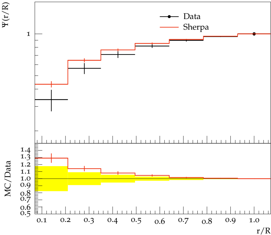
Integral jet shape \Psi for 80 < p_{\perp} < 104
