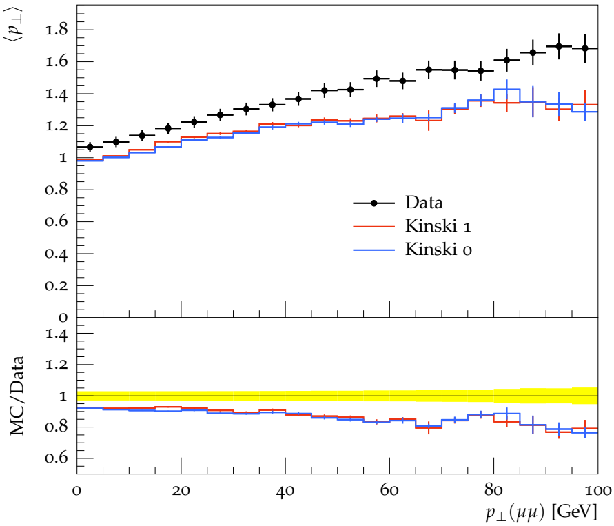
Transverse \langle p_{\perp} \rangle vs p_{\perp}^{\mu\mu}
