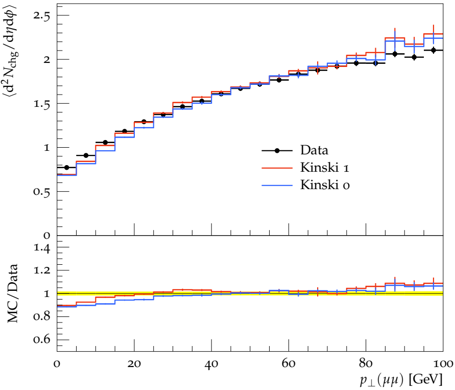
Away N_{\text{chg}} density vs p_{\perp}^{\mu\mu}
