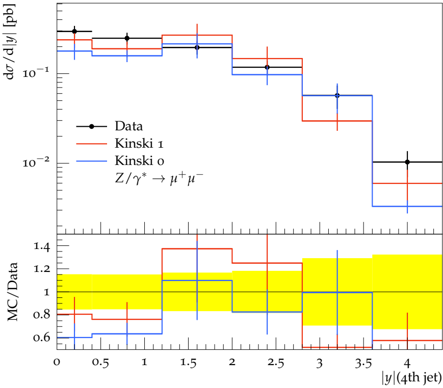
Rapidity of 4th jet
