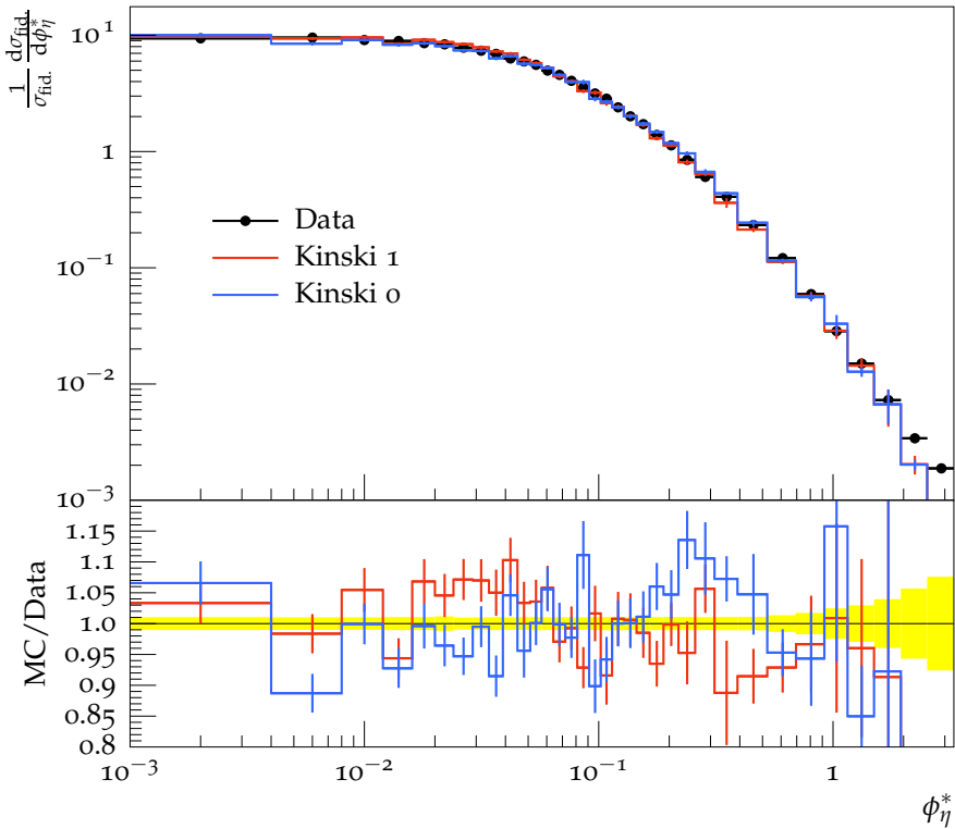
\phi_\eta^* spectrum, Z \rightarrow \mu\mu (dressed), |y_Z| \geq 1.6
