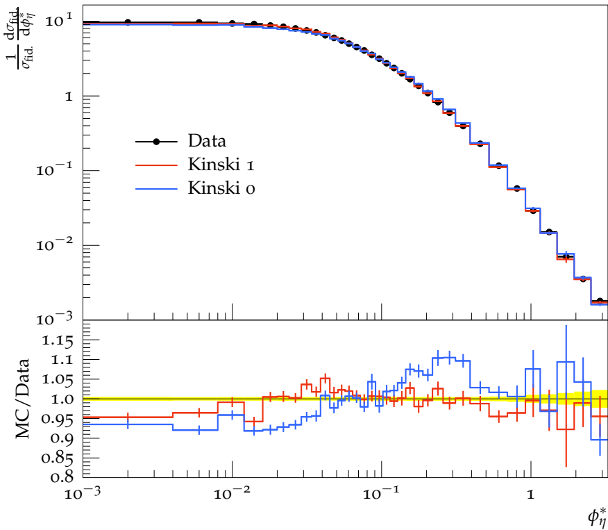
\phi_\eta^* spectrum, Z \rightarrow \mu\mu (bare)
